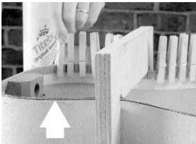
3. The kerfing is installed with 1/64" exposure above the side edges.
