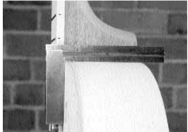
30. Squareness at the top and sides there, and the slight angle of the neck heel, will give you the right action later.
