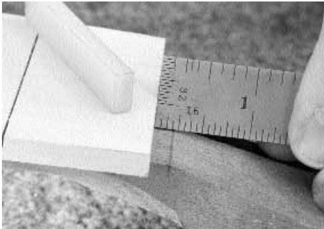
25. The bone nut will rest on the flat area approximately 3/16" to 7/32" wide left between the end of the fingerboard and the break angle of the peghead.
