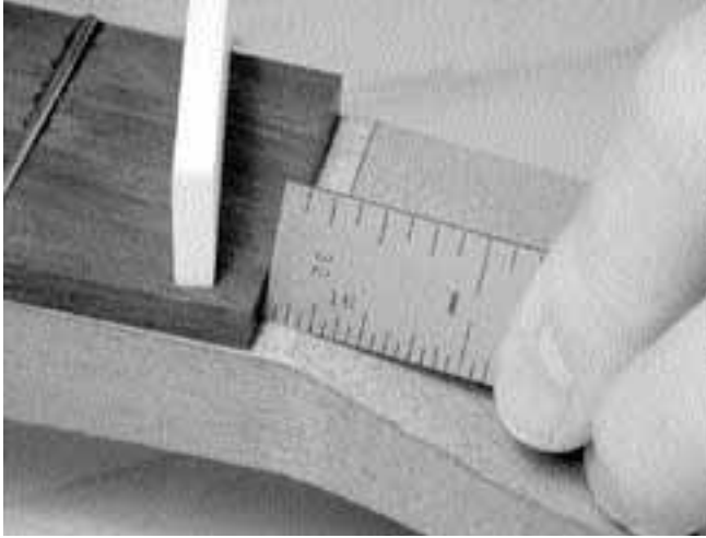
30. The bone nut will rest on the flat area approximately \frac{3}{16} " to \frac{7}{32} " wide, left between the end of the fingerboard and the break angle of the peghead.
