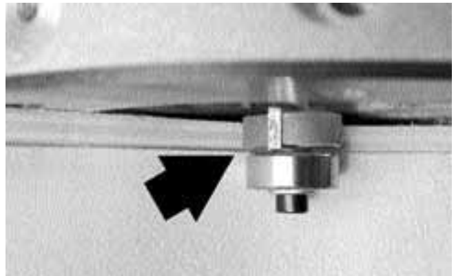
14. Set the height of the router bit cut at 15/64", or slightly more than the thickness of the plywood, so the binding hides the laminated edge of the plywood.
