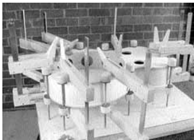
12. A good back clamping setup.
