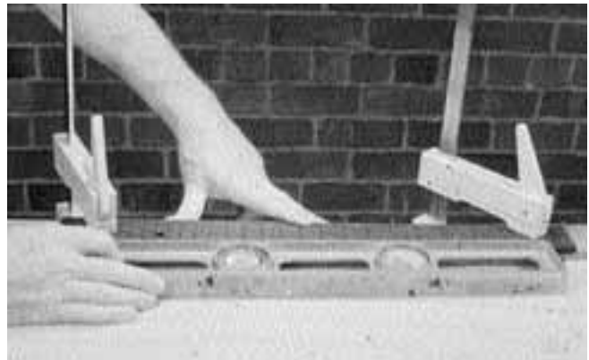
25. Clamped and sanded in this fashion, the fretboard will not only be straight end-to-end, but the edge will be sanded at 90 xxx as well.
